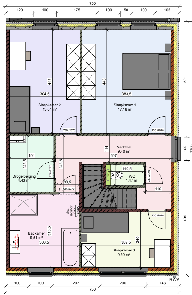
Verdieping LL - lot 6
