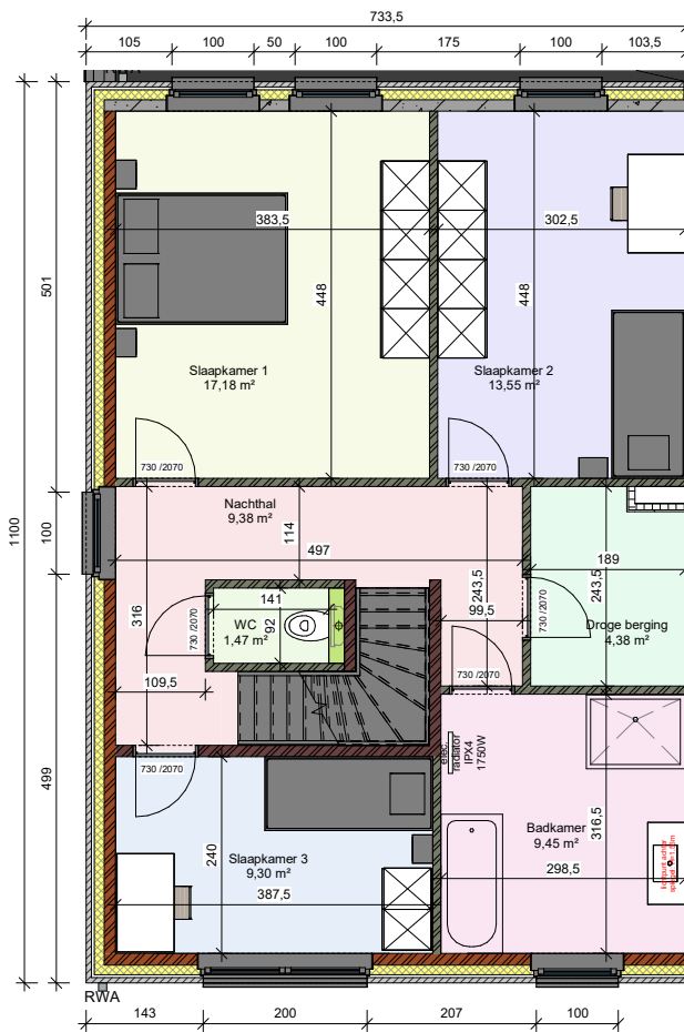
Verdieping LL - lot 1
